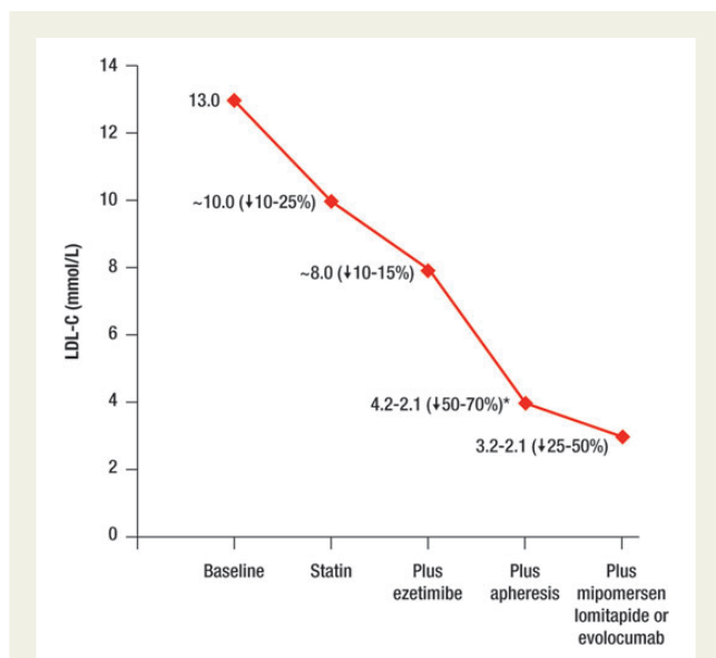
Figure 7 Cumulative low-density lipoprotein cholesterol-lowering effects of statin, ezetimibe, adjunctive mipomersen, lomitapide or evolocumab, and lipoprotein apheresis in homozygous familial hypercholesterolaemia. The per cent low-density lipoprotein cholesterol reduction is dependent on baseline low-density lipoprotein cholesterol values. *The figure illustrates the decrease in low-density lipoprotein cholesterol after a single apheresis treatment. The low-density lipoprotein cholesterol level achieved after treatment is higher in patients with higher baseline value. However, the rebound curves after treatment are more or less parallel. See Schuff-Werner et al. 43
